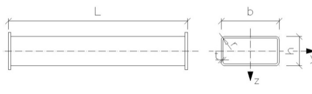
Figure 2. Scheme of the test members; group B
