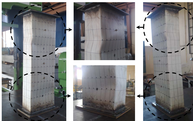
Figure 4. Test completion and overall failure; member B22
